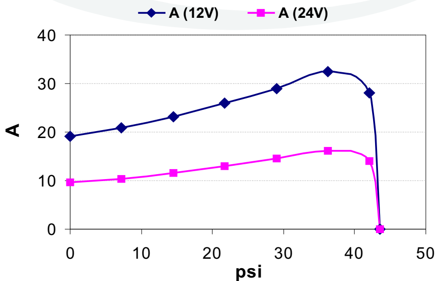
AMPERE-DRAW DIAGRAM
