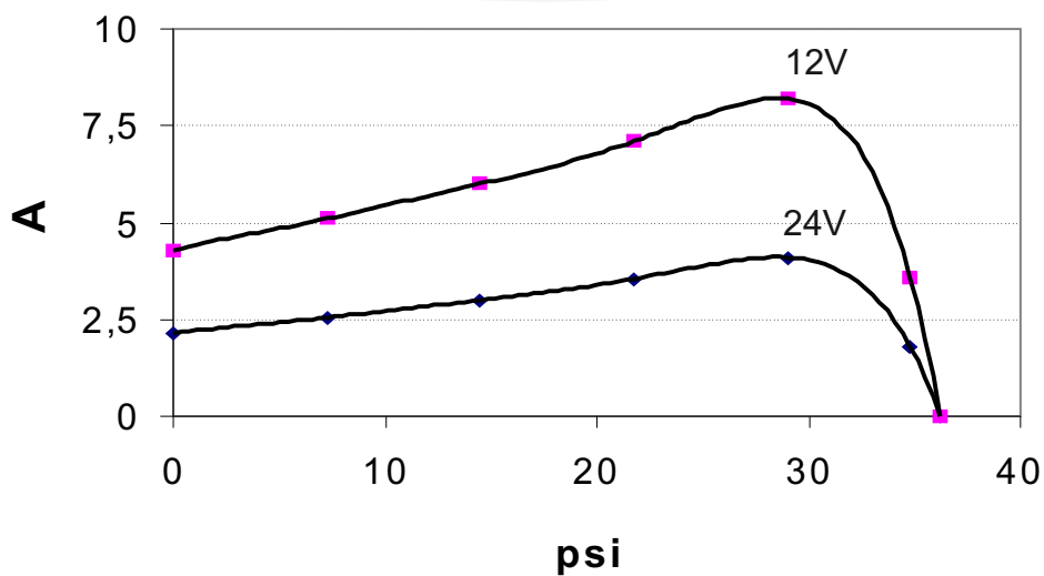
AMPERE-DRAW DIAGRAM
