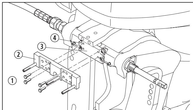
6 Attaching Mounting Brackets on BRP Engines
