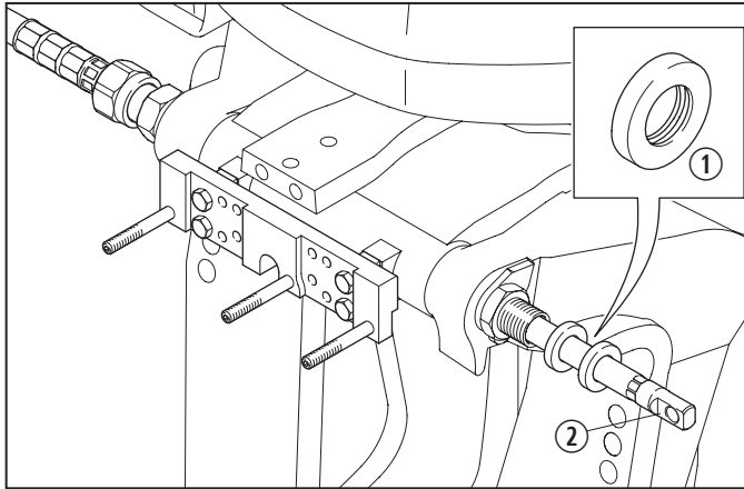
7 Attaching the Retraction Spacers
