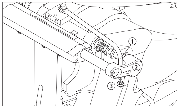
12 Securing the Engine Link Arm
