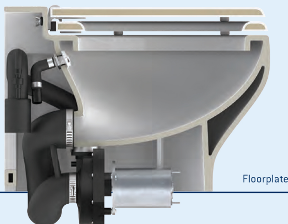
Cross section Silence Plus 2G Short, Deep Bowl (Through Floor Installation)
